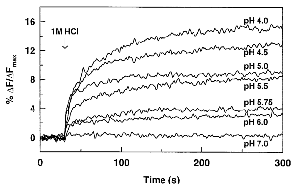
Fig. 4. Effect of pH on lipid mixing for 5 mol% Lipo-AcE4K in POPC LUVs. Lipopeptide was added from a 2 mM DMSO stock solution to a 1:3 mixture of labelled and unlabelled vesicles prior to the addition of 1M HCl to achieve the indicated pH.
