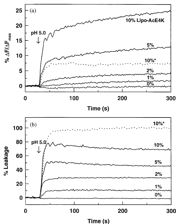
Fig. 7. Lipid mixing and leakage in EPC/Chol (55:45) LUVs. (a) 0 to 10 mol% Lipo-AcE4K was added to a 1:3 mixture of labelled and unlabelled vesicles (0.2 mM total lipid) from a 2 mM stock solution in DMSO. Lipid mixing assays were as described above, adding 1 M HCl at 30 s to achieve a final pH of 5.0. (b) Leakage assays for 0 to 10 mol% Lipo-AcE4K added to liposomes containing 6 mM ANTS and 75 mM DPX. * For comparison, corresponding assays for 10 mol% Lipo-AcE4K in EPC LUVs are shown (dotted lines).
